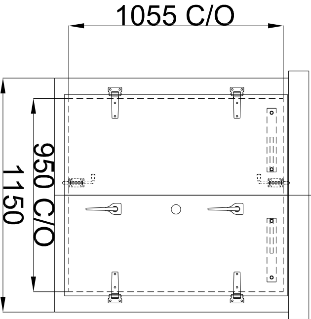
EXTERNAL VIEW ON FRONT WALL
