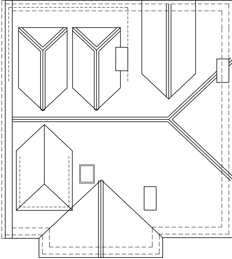
Roof Plan
