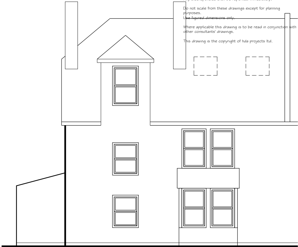
South Elevation
