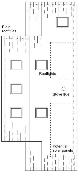
Roof Plan
