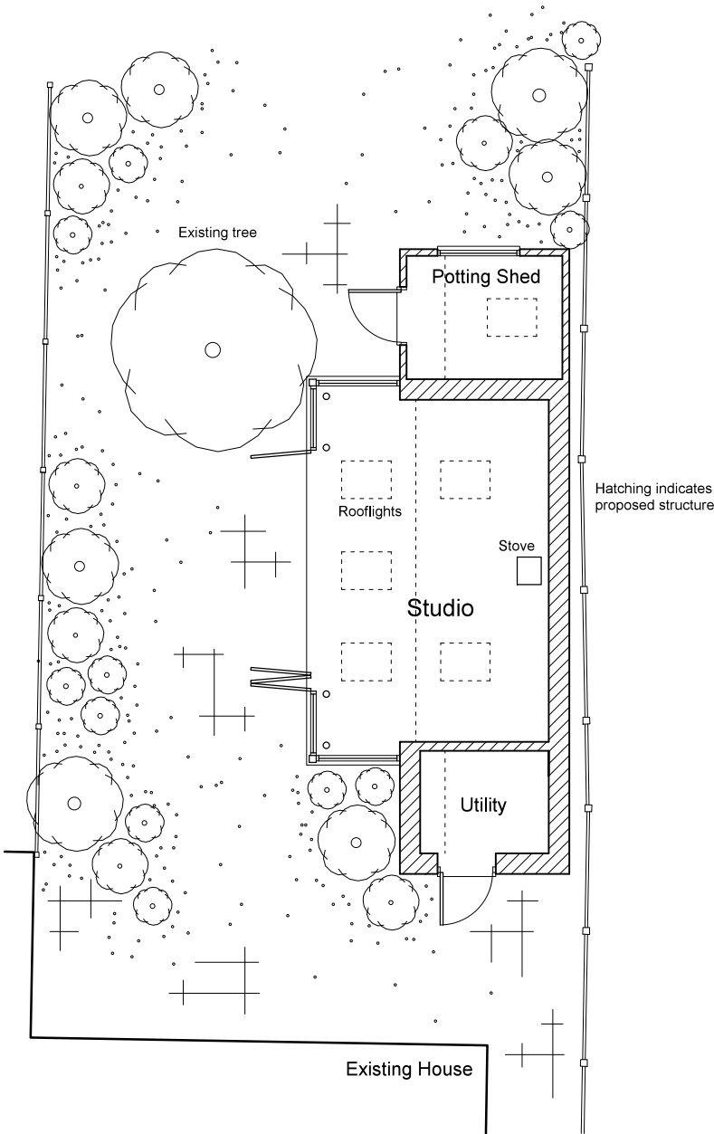
Floor Plan
