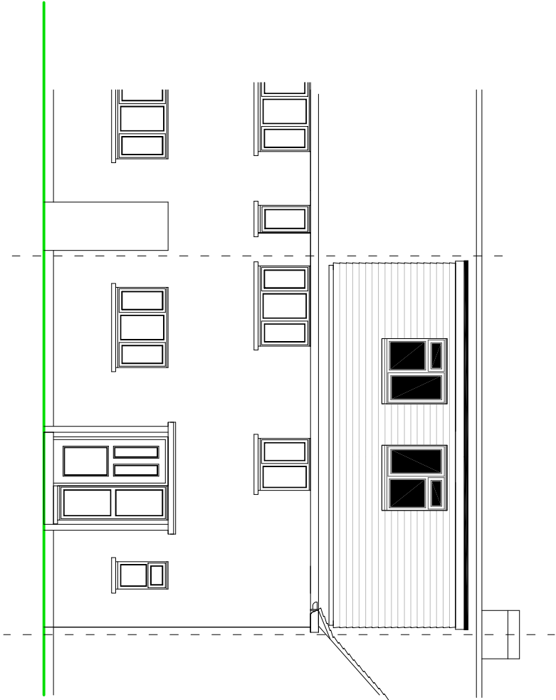
FRONT (EAST) ELEVATION
