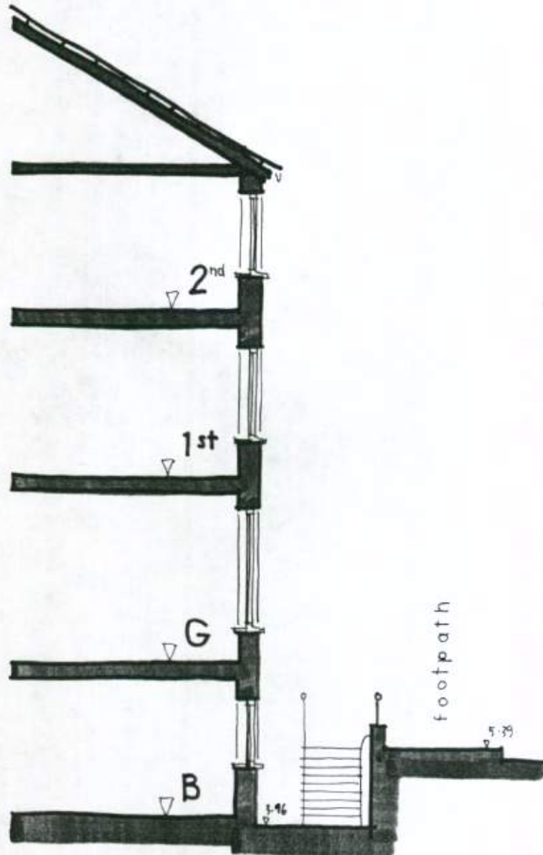
SECTION THRO' 1:100
