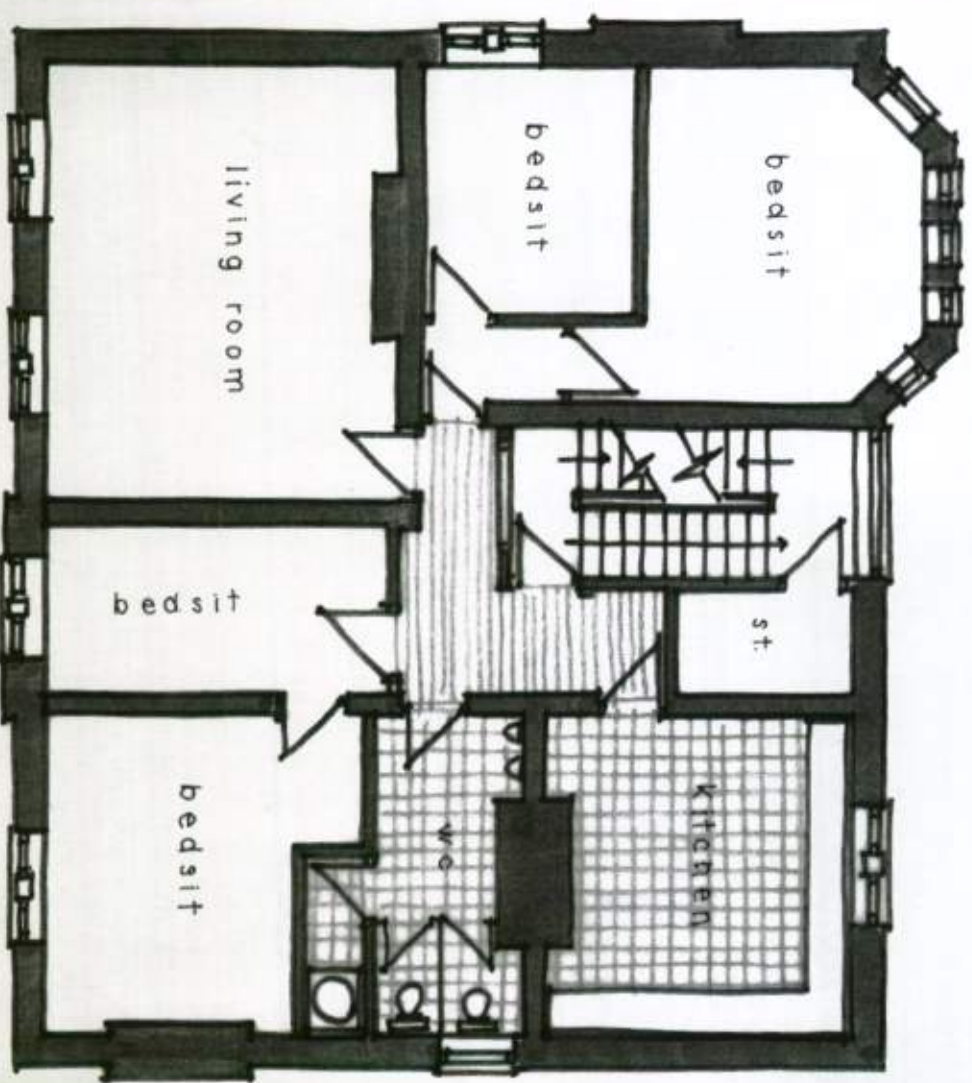
1st FLOOR PLAN 1:100
