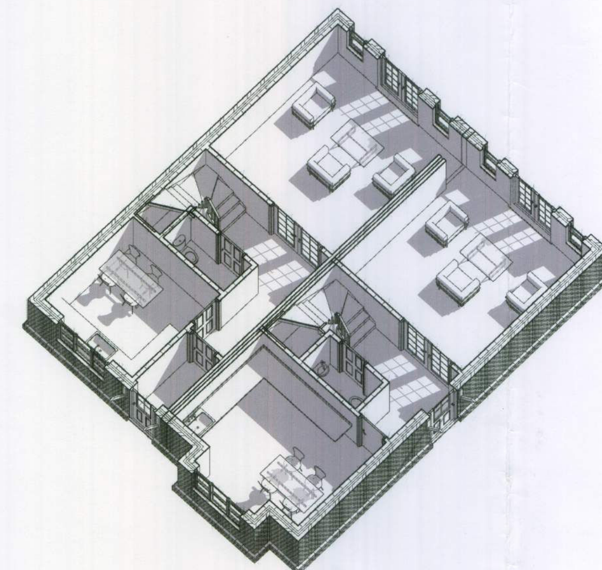
8 Ground Floor Axonometric
