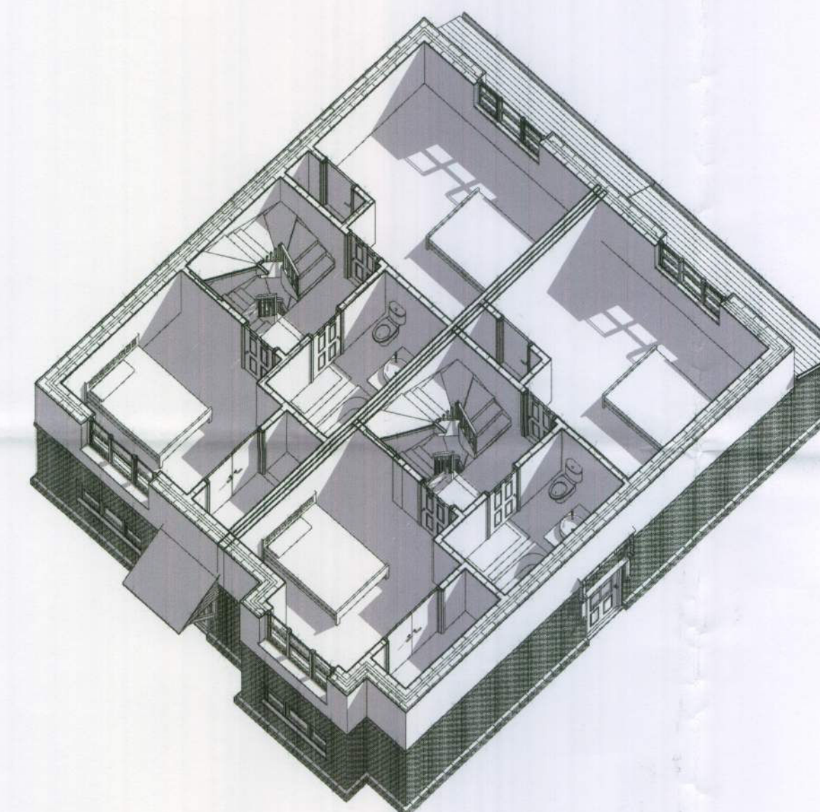
9 First Floor Axonometric
