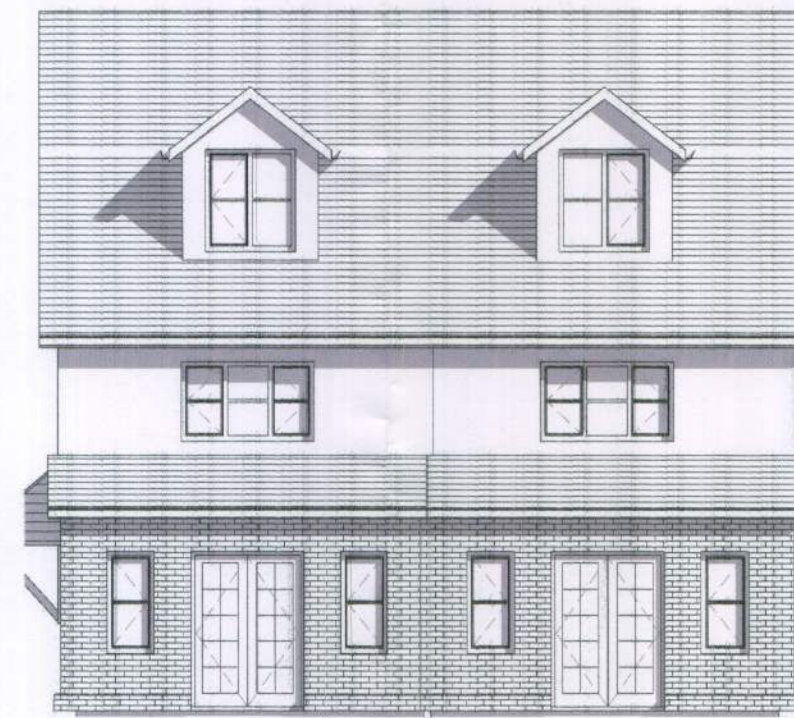
5 South 1:100
