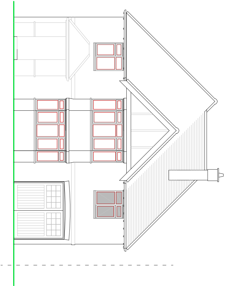
FRONT ELEVATION
