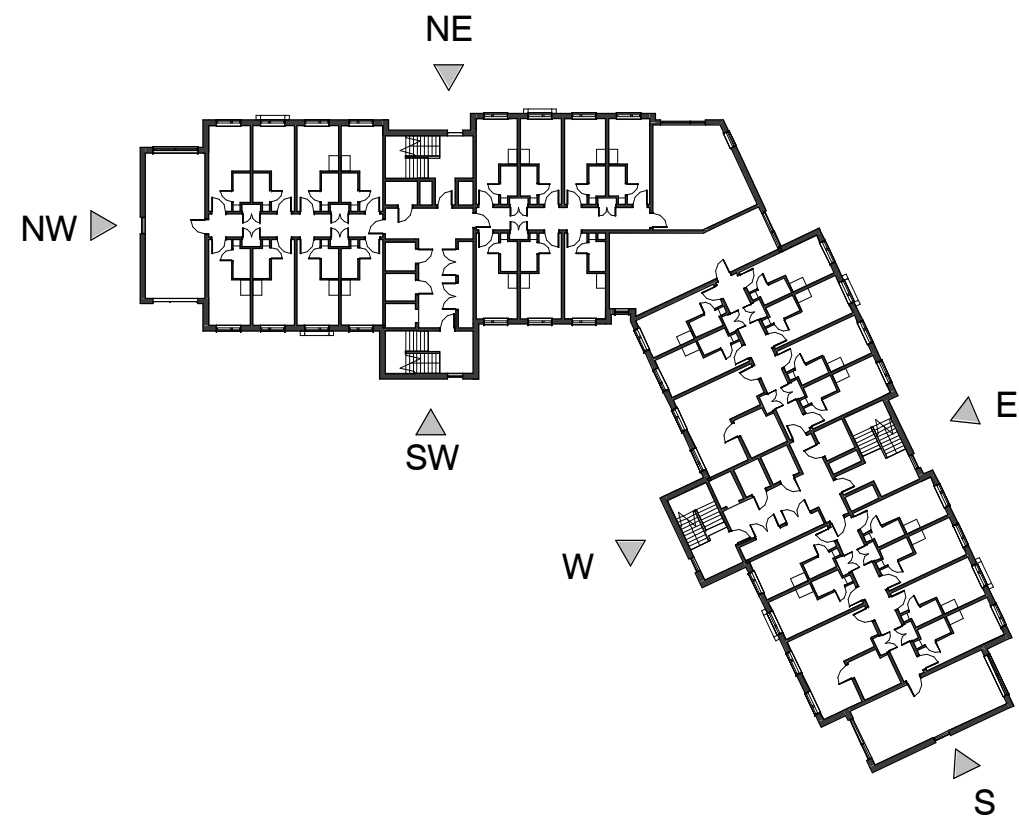
First Floor Plan 1:500
