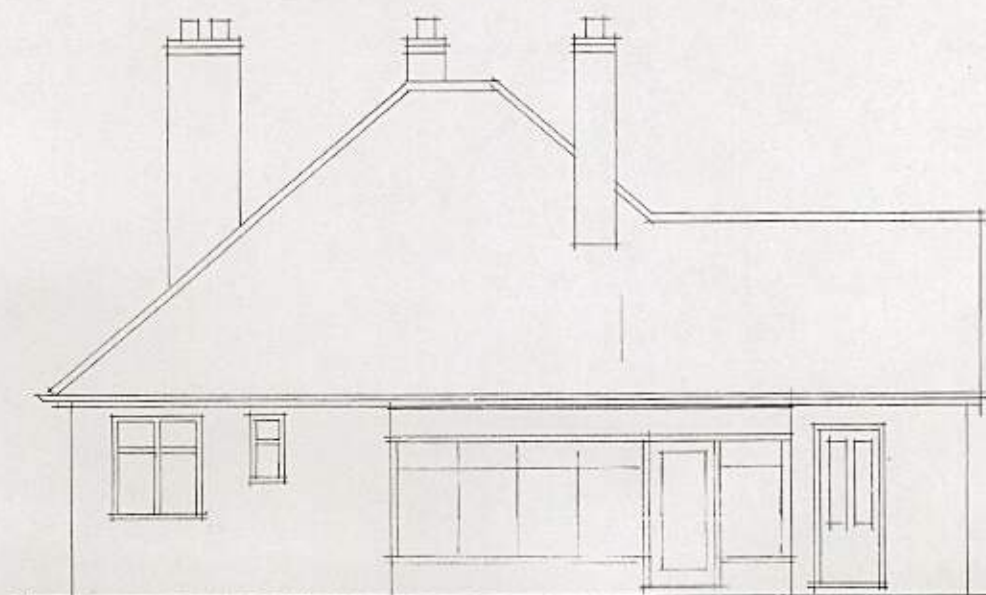
REAR ELEVATION
