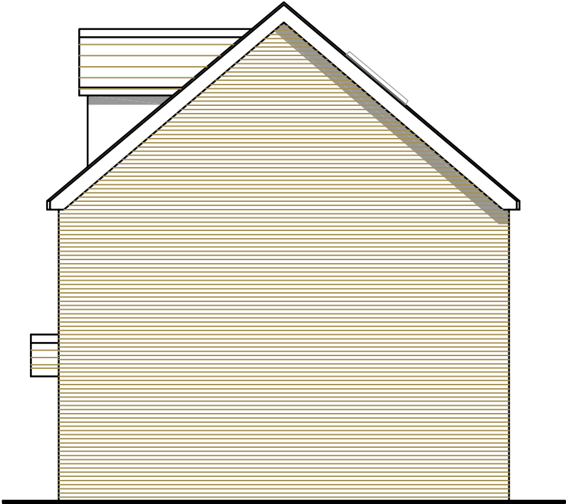
Side (North Unit 3) Elevation
