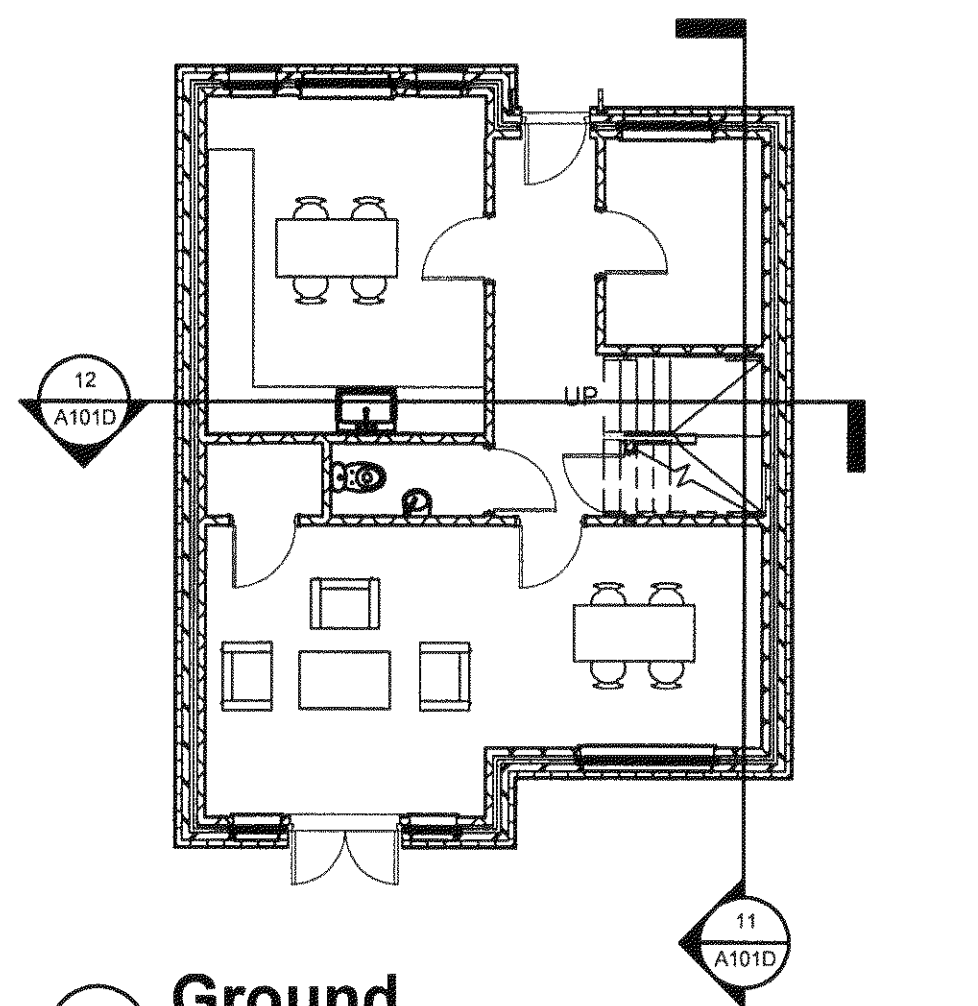
1 Ground 1 : 100
