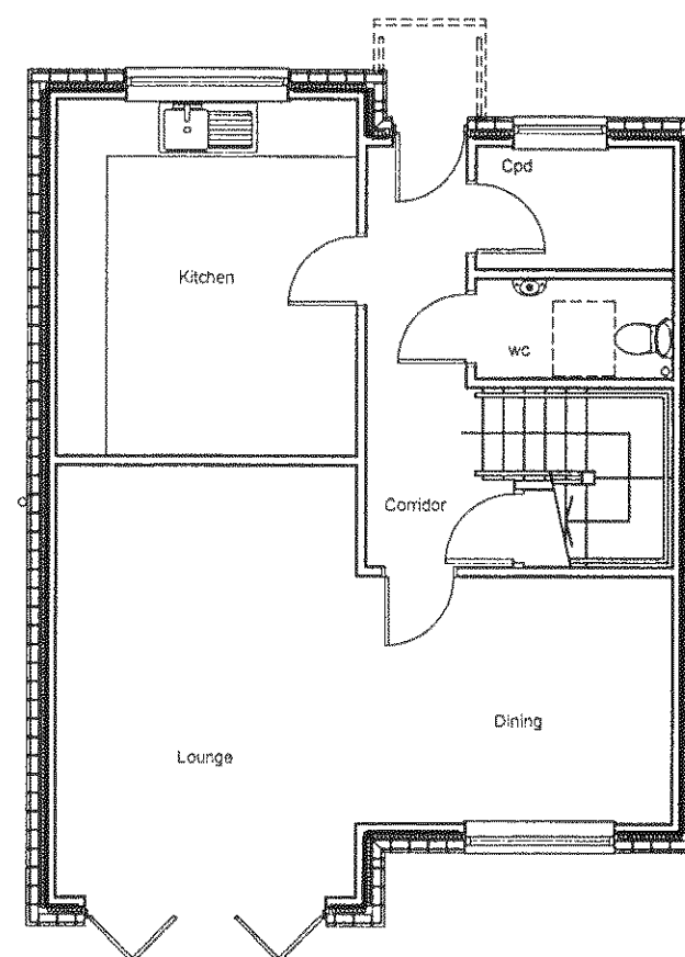
A Ground 1 : 100
