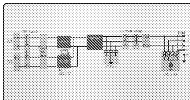
Growatt TL3-S block diagram
