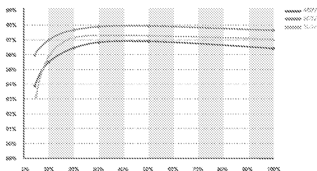
Growatt TL3-S efficiency
