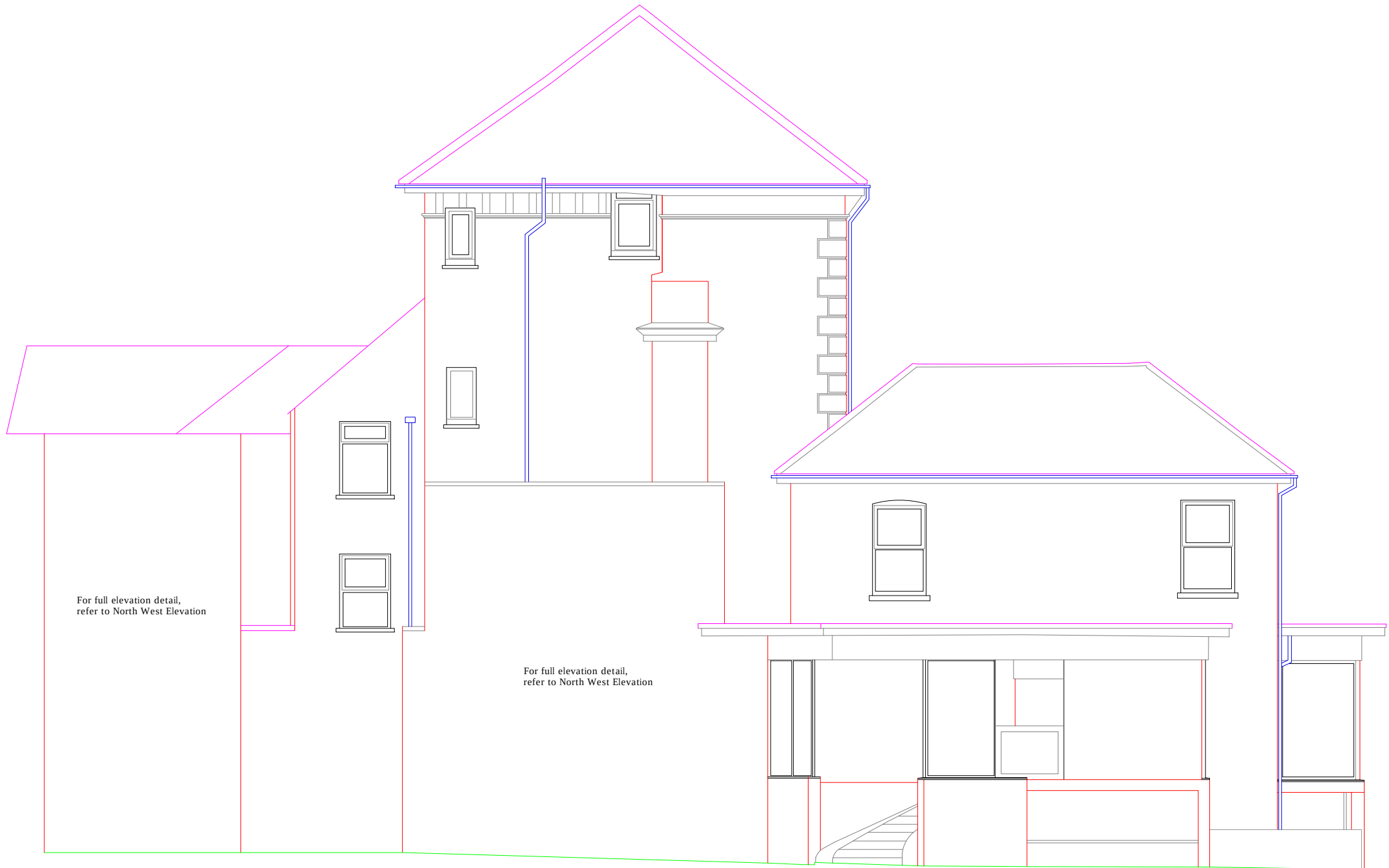
WEST ELEVATION
