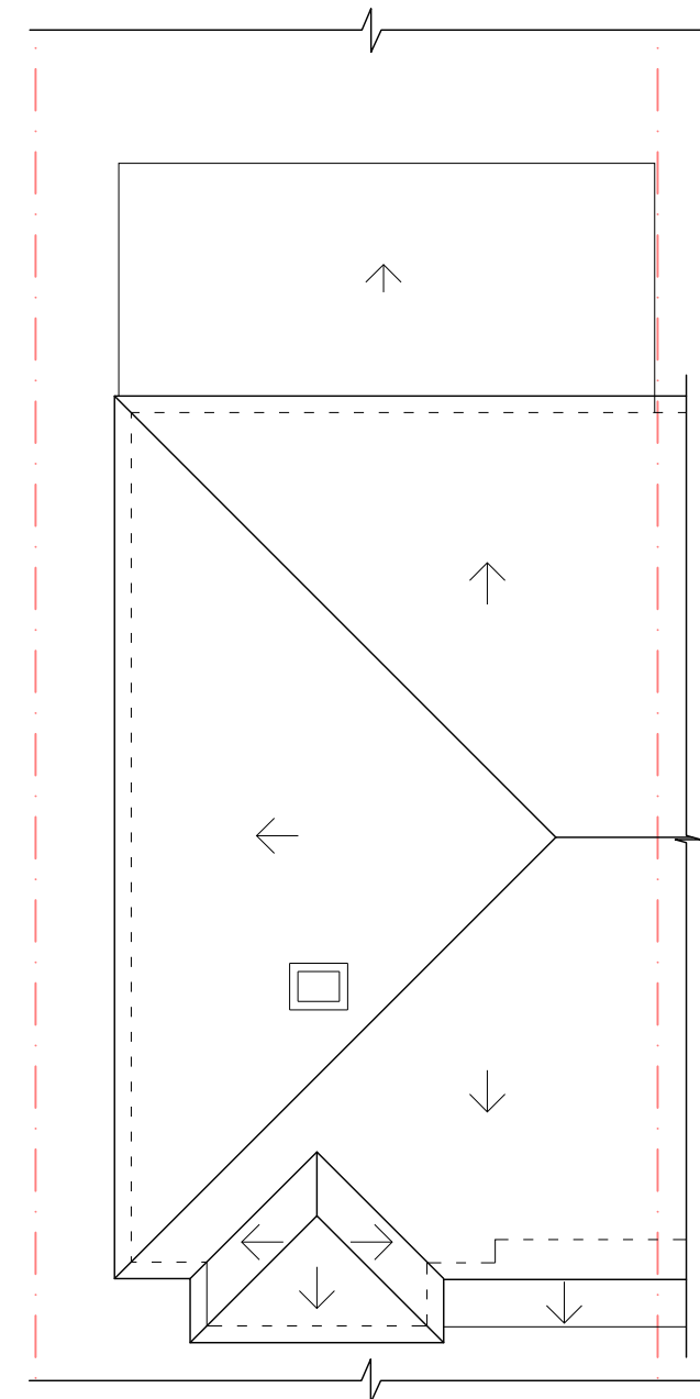
PROPOSED ROOF PLAN, Sc. 1:100
