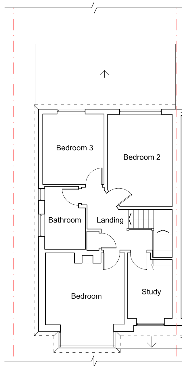
PROPOSED FIRST FLOOR PLAN, Sc. 1:100
