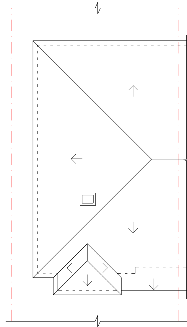
EXISTING ROOF PLAN, Sc. 1:100
