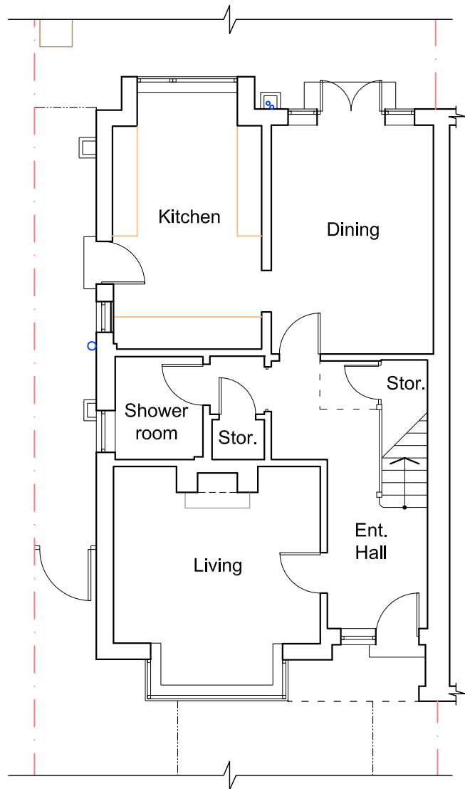
EXISTING GROUND FLOOR PLAN, Sc. 1:100
