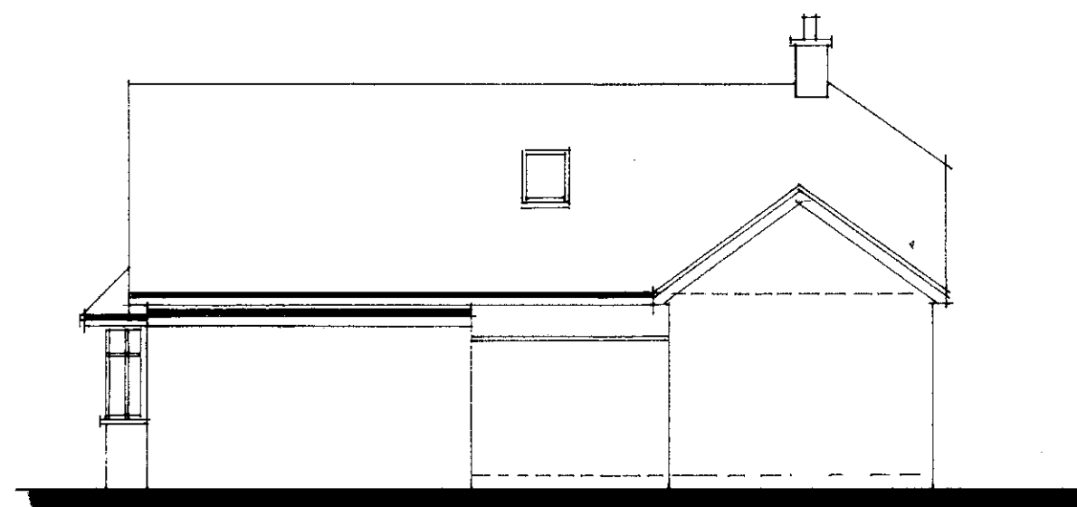
WEST ELEVATION
