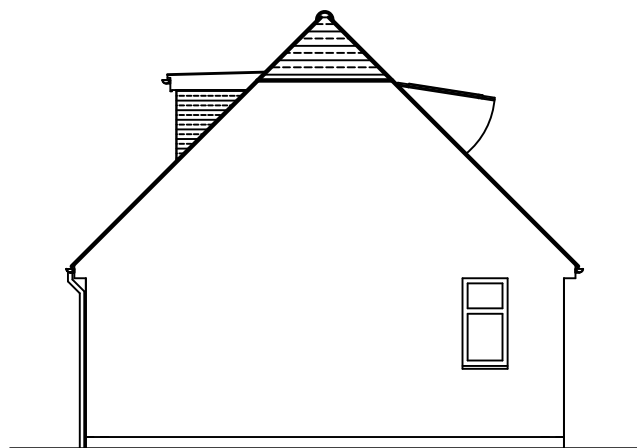
Proposed Side Elevation (West)
