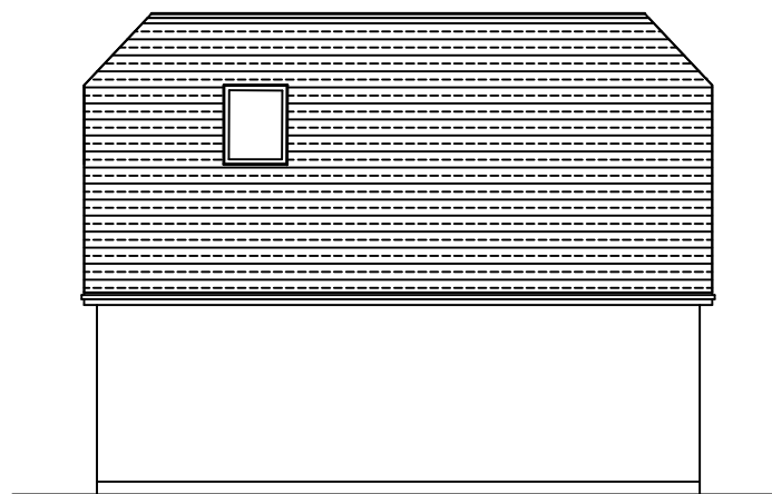
Proposed Rear Elevation (South)
