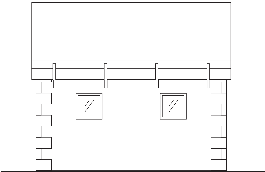
SIDE D 1:50
