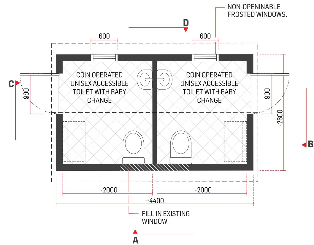
AMENITIES - DETAIL PLAN 1:50 @ A3
