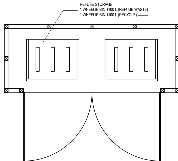
REFUSE: PLAN SCALE : 1:50 @ A3
