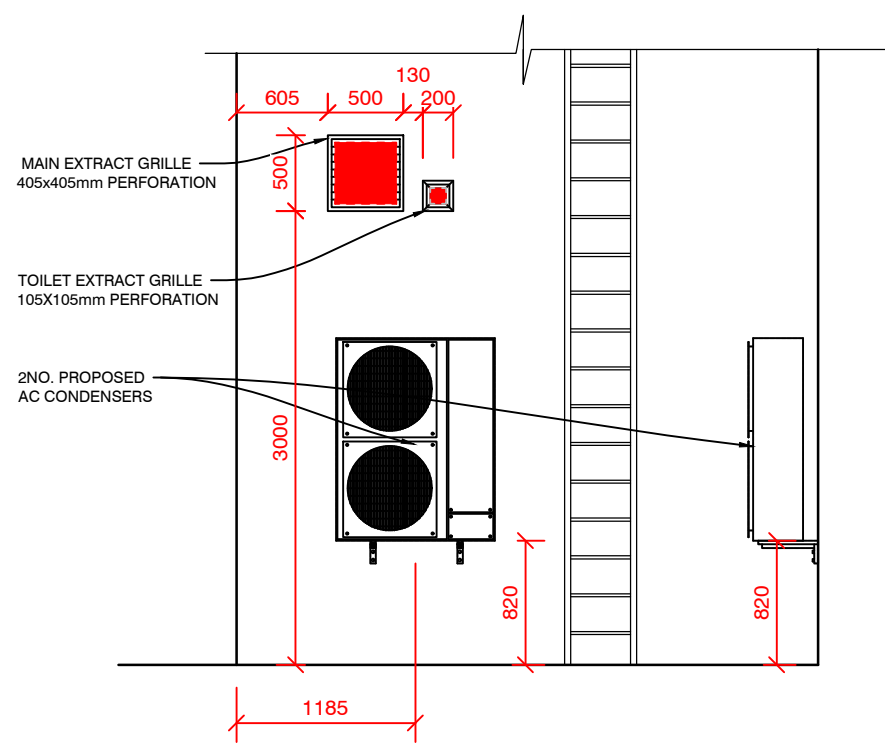
PROPOSED LH SECTION THRO'
