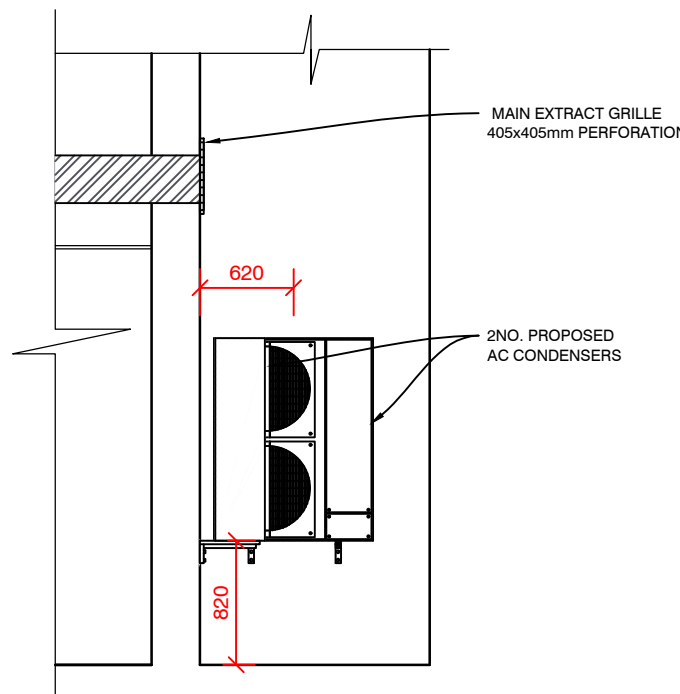
PROPOSED RH SECTION THRO'
