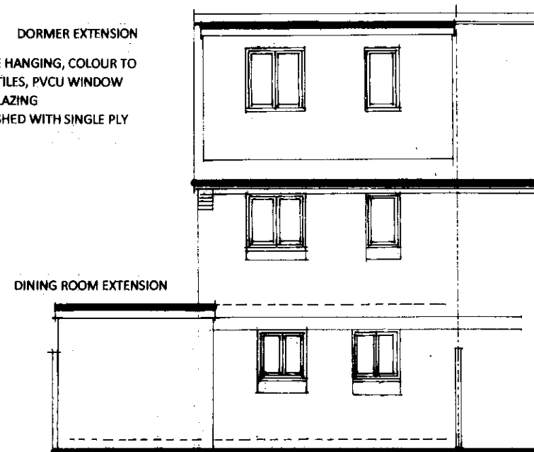
EAST ELEVATION TO REAR GARDEN
