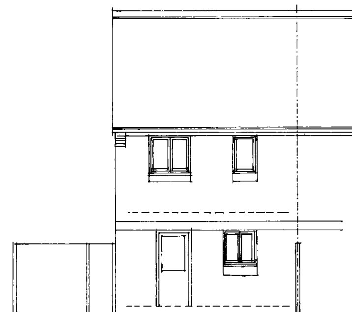
EAST ELEVATION TO REAR GARDEN
