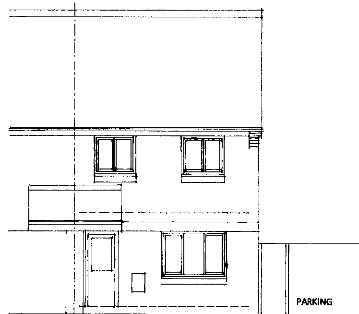
WEST ELEVATION TO KEW GARDENS
