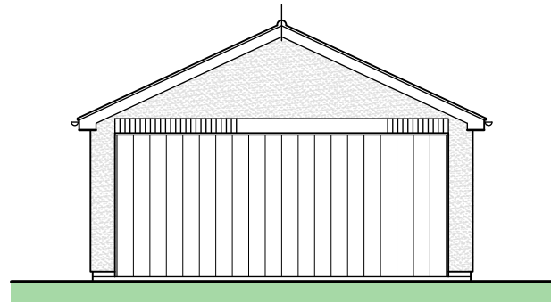
FRONT ELEVATION EAST
