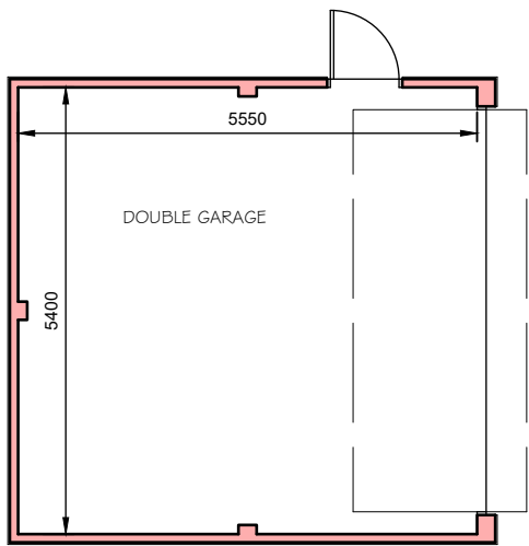
FLOOR PLAN
