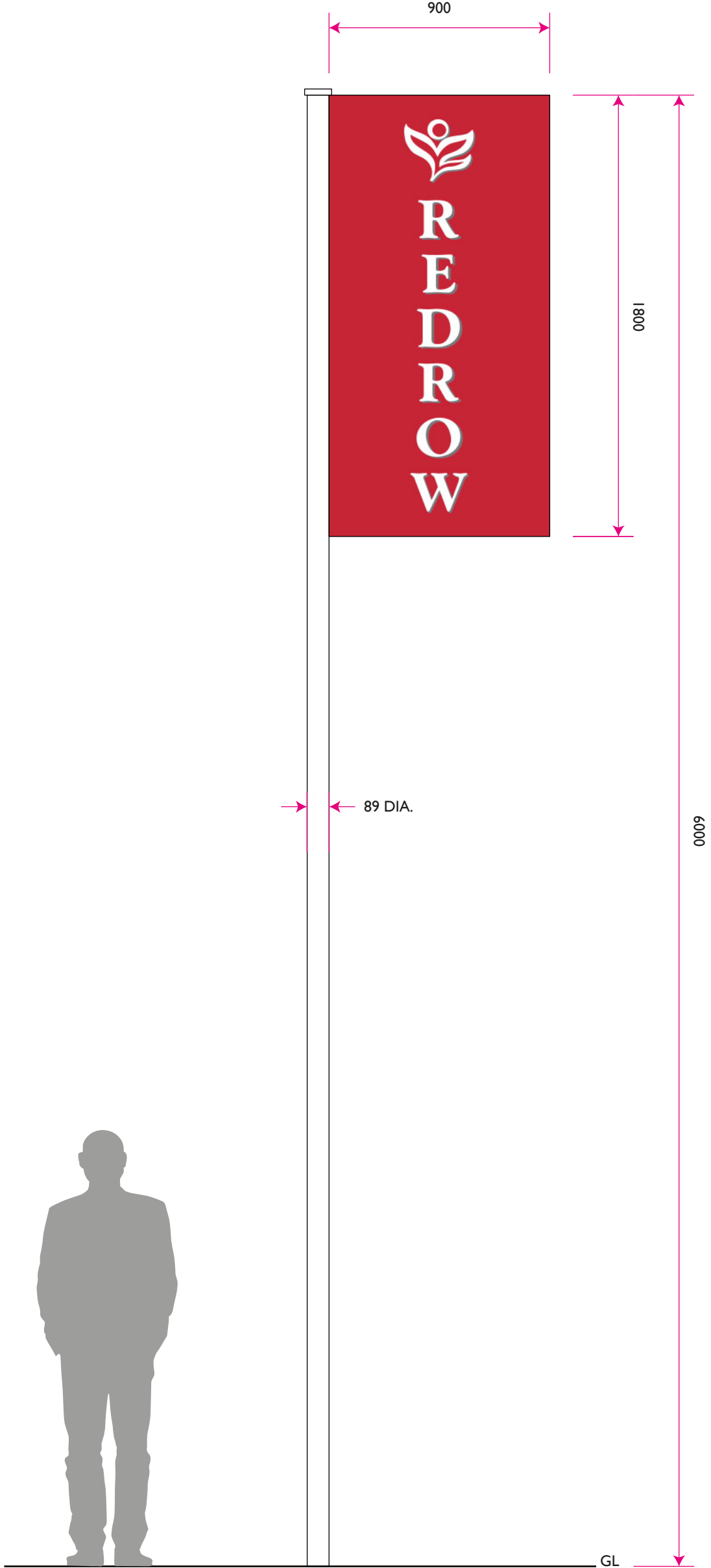
Front Elevation - Scale - 1/20@A2 all dimensions in mm
