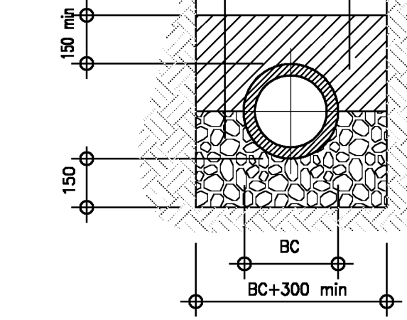
CLASS B BEDDING
