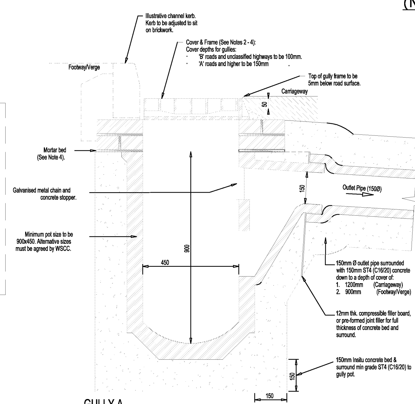
GULLY A TYPE: PRECAST CONCRETE SECTION (1:10)
