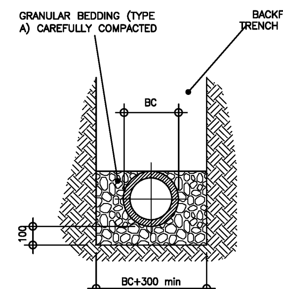
GRANULAR SIDE FILL TO BE USED WHERE COVER TO CROWN OF PIPE IS GREATER THAN 900mm UNDER ROADS, FOOTWAYS & HARDSTANDINGS
