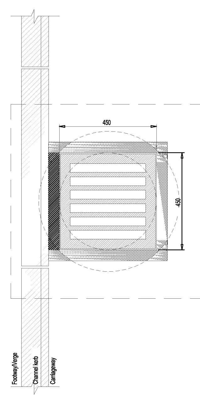
GULLY A TYPE: PRECAST CONCRETE PLAN (1:10)
