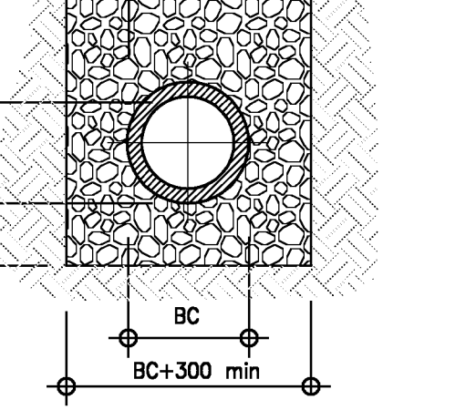
CLASS S BEDDING
