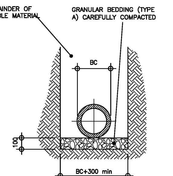
GRANULAR BED TO BE USED WHERE COVER TO CROWN OF PIPE IS GREATER THAN 900mm IN LANDSCAPED AREAS
