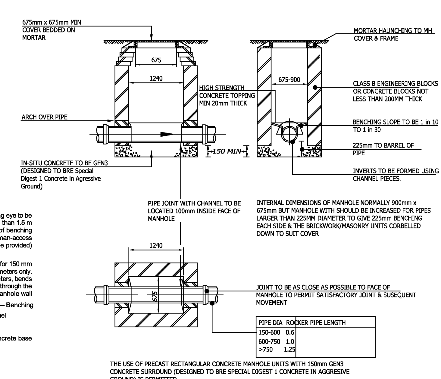
FIG 2.7 SFA 6 - MANHOLE TYPE D DEPTH TO SOFFIT <1M (NTS)
