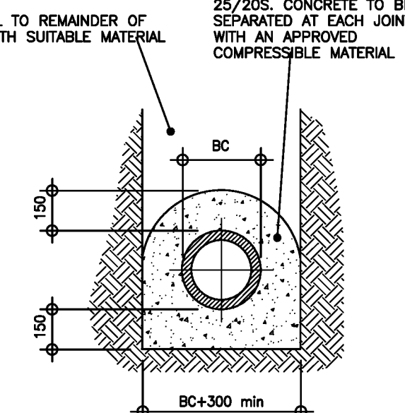
CONCRETE SURROUND TO BE USED WHERE COVER TO CROWN OF PIPE IS LESS THAN 900mm UNDER ROADS, FOOTWAYS & HARDSTANDINGS AND LESS THAN 600mm IN LANDSCAPED AREAS
