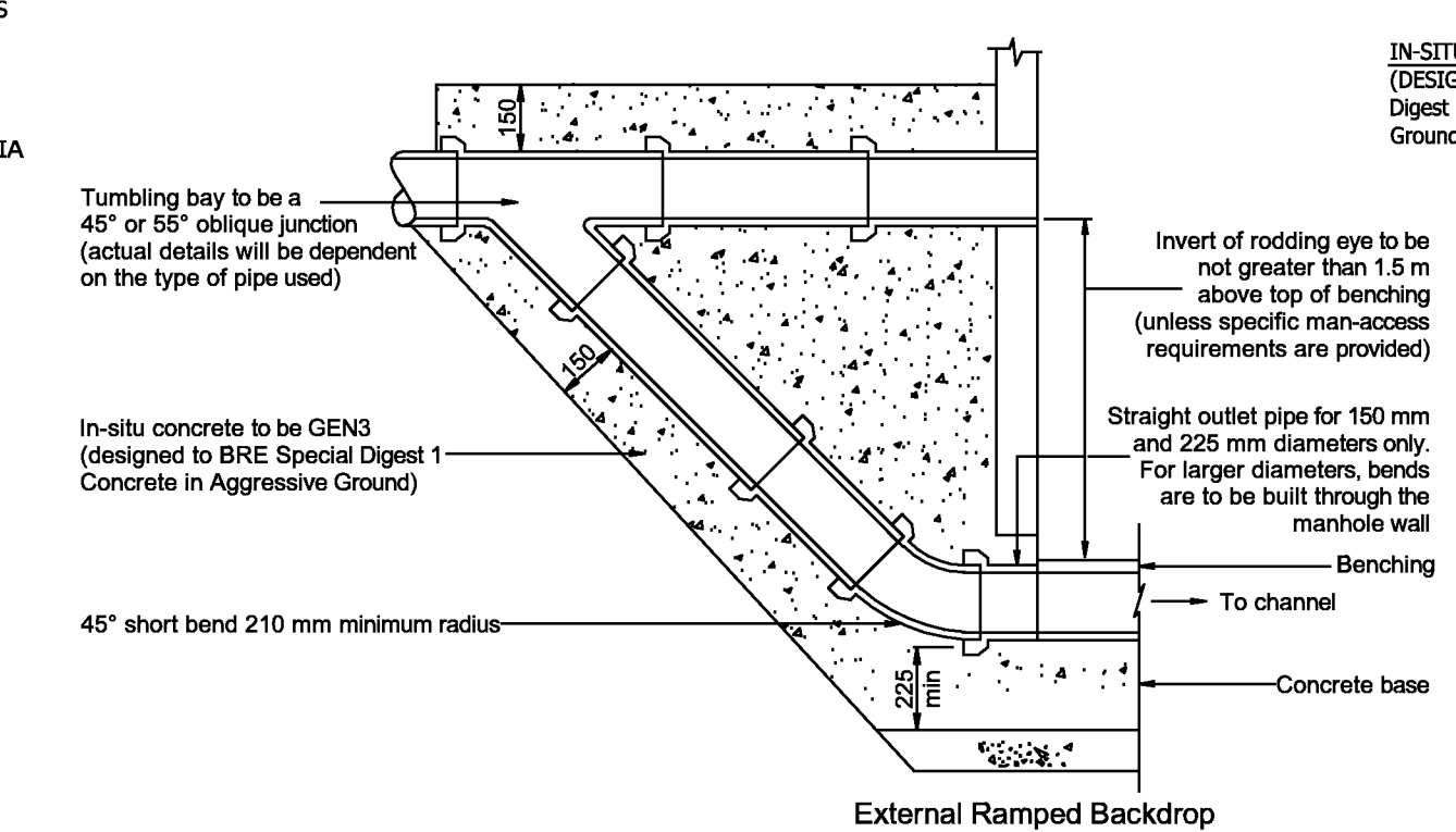
FIG 2.10 SFA 6 - EXTERNAL RAMPED BACKDROP
