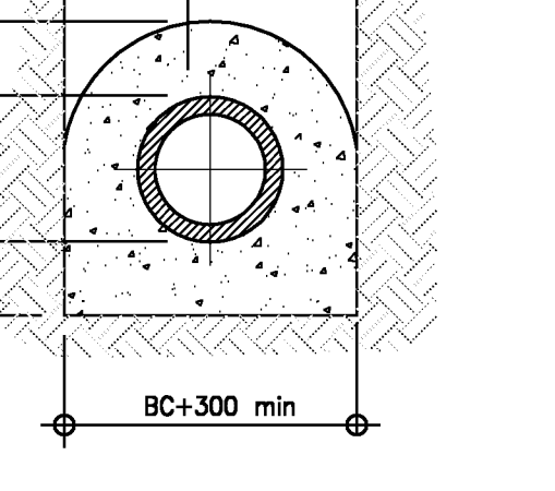
CLASS Z BEDDING
