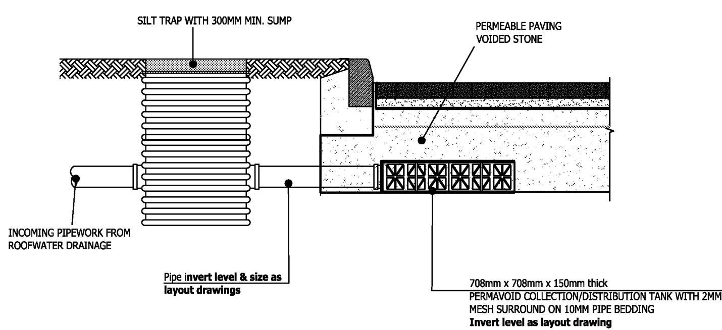
TYPICAL POROUS INLET DETAIL (MARKED DT ON LAYOUT)
