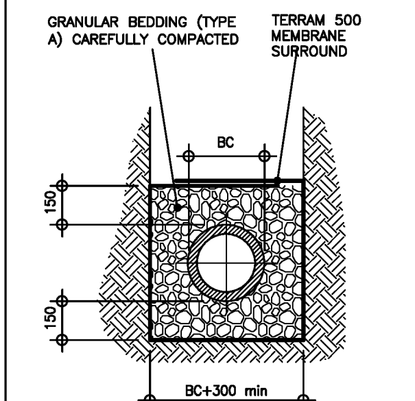
GRANULAR SURROUND TO BE USED WHERE PIPE PASSES WITHIN 3M OF NEW OR EXISTING TREES UNLESS PIPE REQUIRED CONCRETE SURROUND
