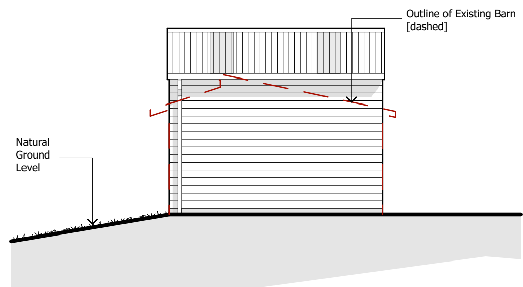
PROPOSED NORTH - WEST ELEVATION [1:100]
