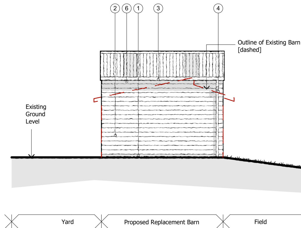
PROPOSED SOUTH - EAST ELEVATION [1:100]
