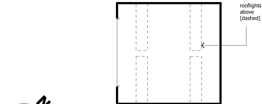
PROPOSED PLAN [1:100]
