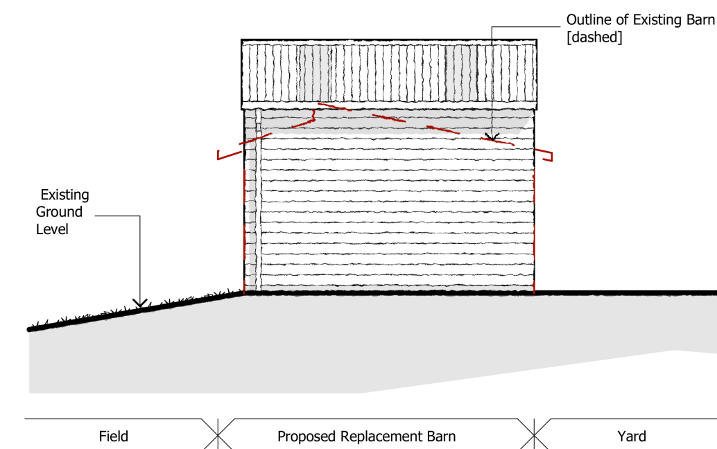
PROPOSED NORTH - WEST ELEVATION [1:100]
