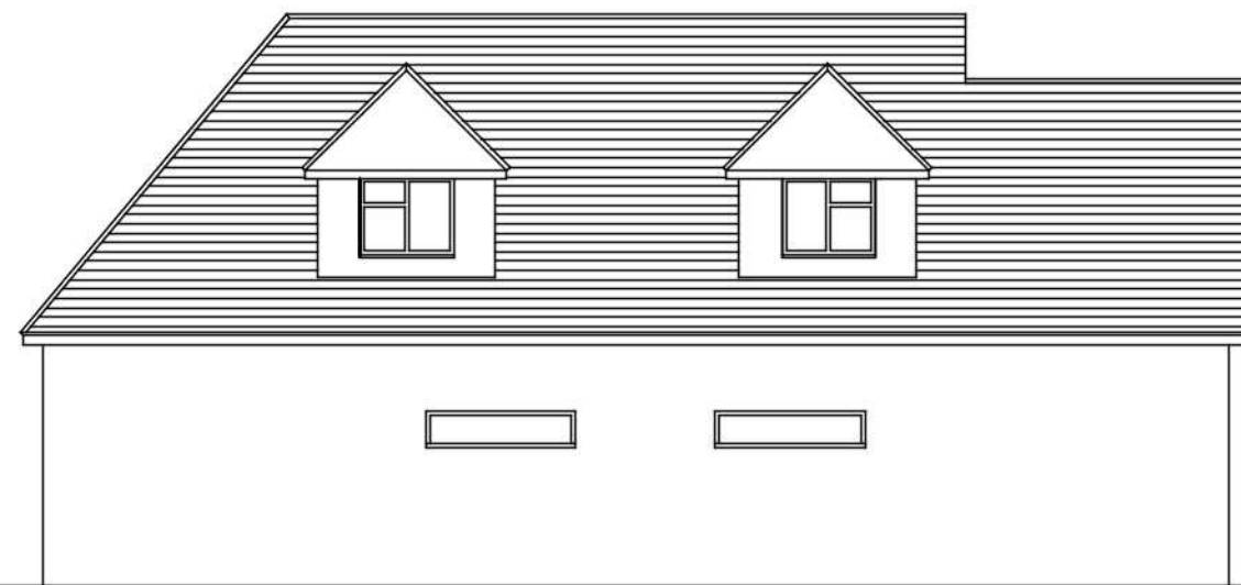
Proposed East (Rear ) Elevation
