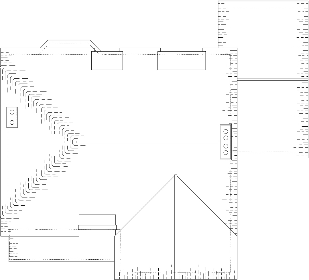
Roof Plan Proposed
