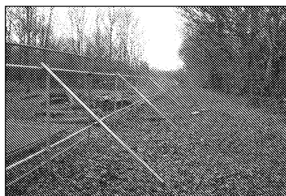
Photo 2: Heras fencing wired to scaffold braced posts is a robust and effective interpretation of the BS specification.
