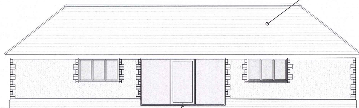
Proposed West Elevation 1:100
