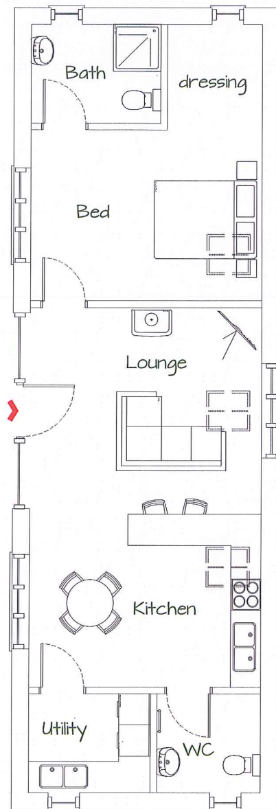
Proposed Plan 1:100
