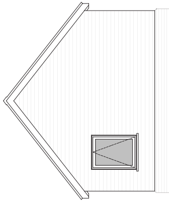
Approved South Elevation 1:100
