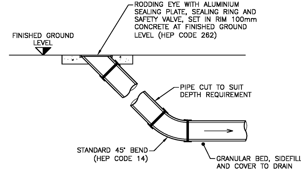
RODDING EYE DETAIL (VC SHOWN – PVCu ALTERNATIVE TO SUIT) (1:25)
