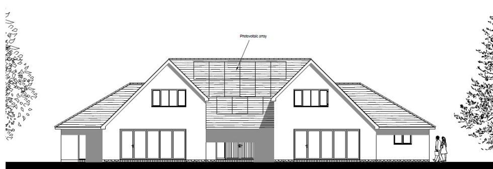
FRONT (SOUTH) ELEVATION
