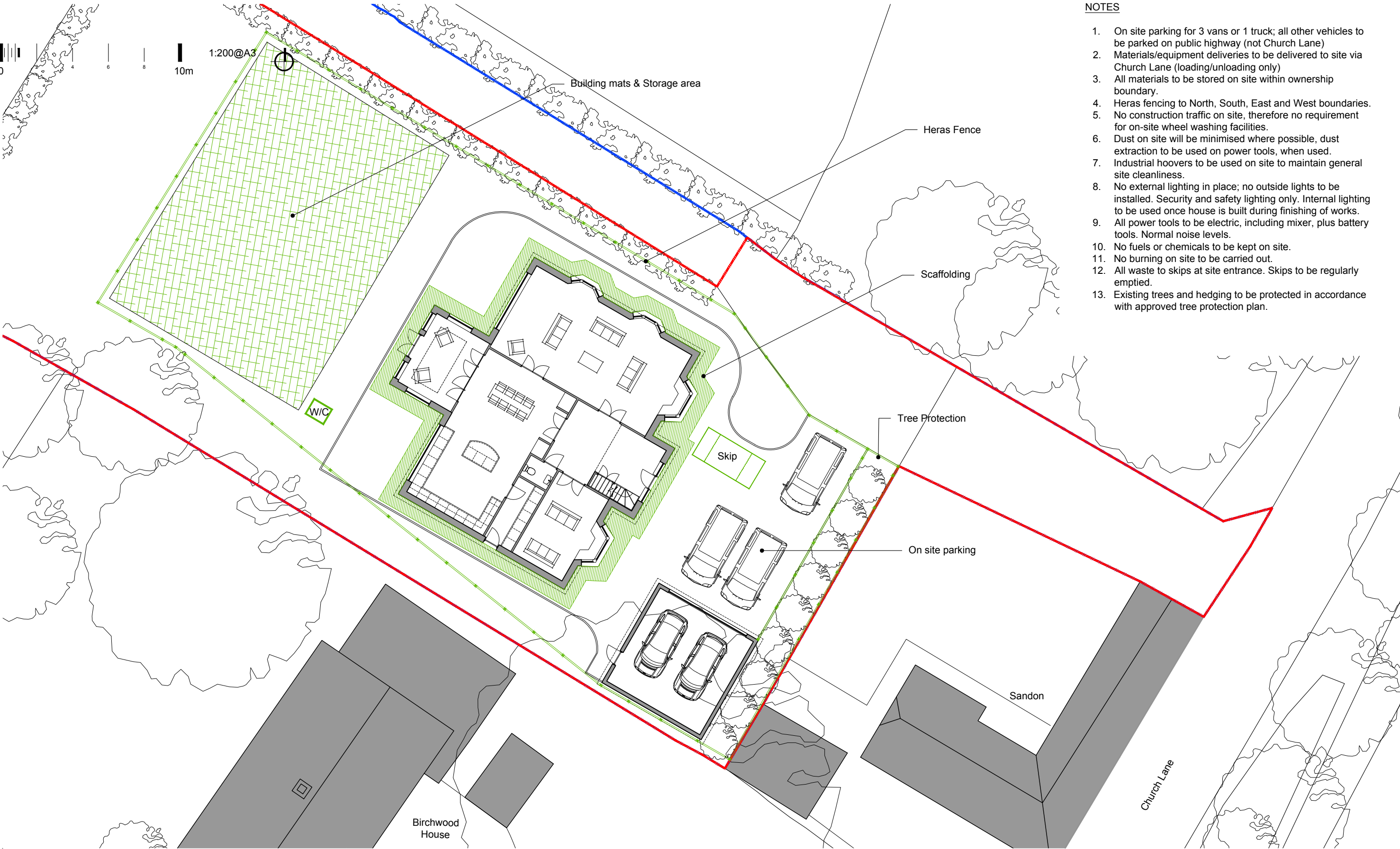
Site Layout Plan - Site set-up during construction
