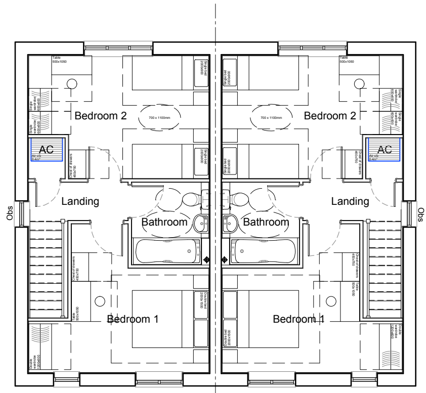
First Floor Plan *Obs - Obscured Glass
