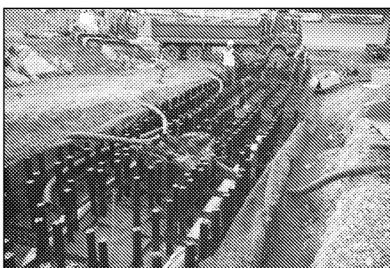
Photo 55: The individual Silva Cells can be assembled in layers and service ducting threaded through before filling with soil and fitting the reinforced tops.
