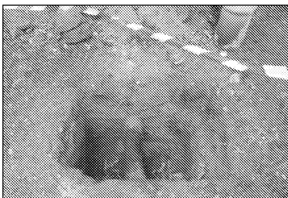
Photo 38: Where piles are proposed close to trunks, it is essential to excavate 50–75cm deep to see if there are any significant roots in the way, with provision to move the pile location if roots are found (note the pile was finally installed to avoid this root).
