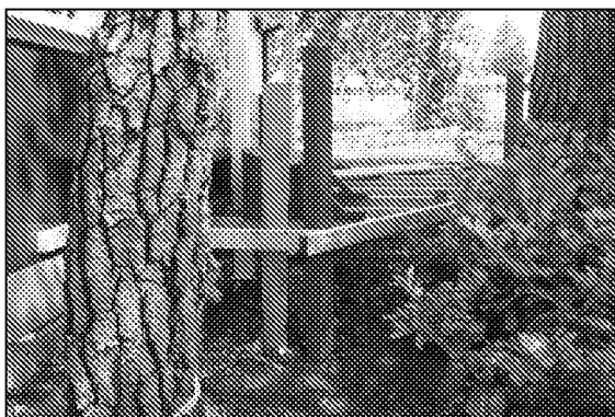
Photo 32: New surfacing can be supported above the ground on posts leaving the soil surface beneath undisturbed.
