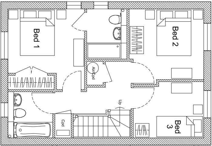
PLOT 3 FIRST FLOOR
