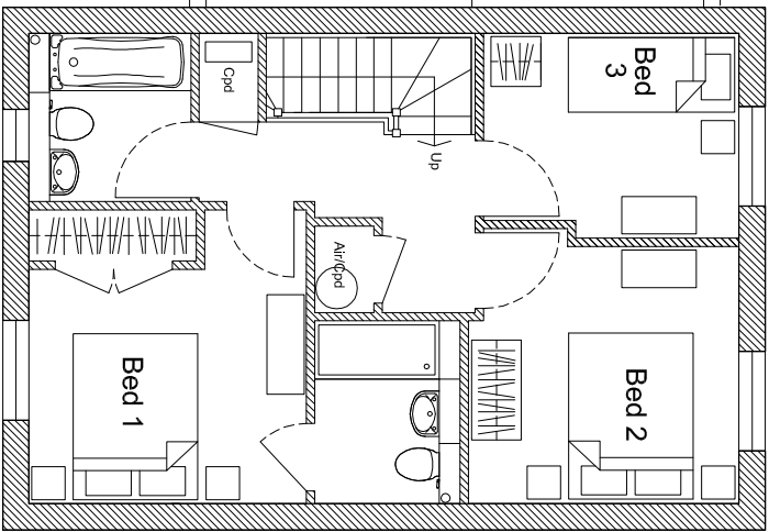
PLOT 4 FIRST FLOOR
