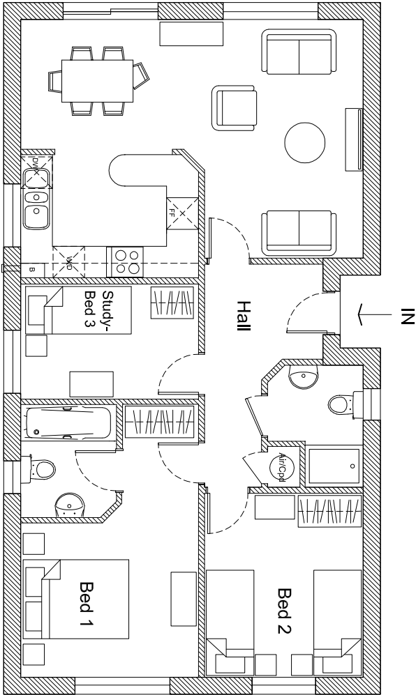
PLOT 2 GROUND FLOOR
