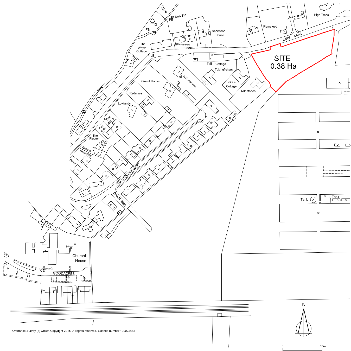
Location Plan
