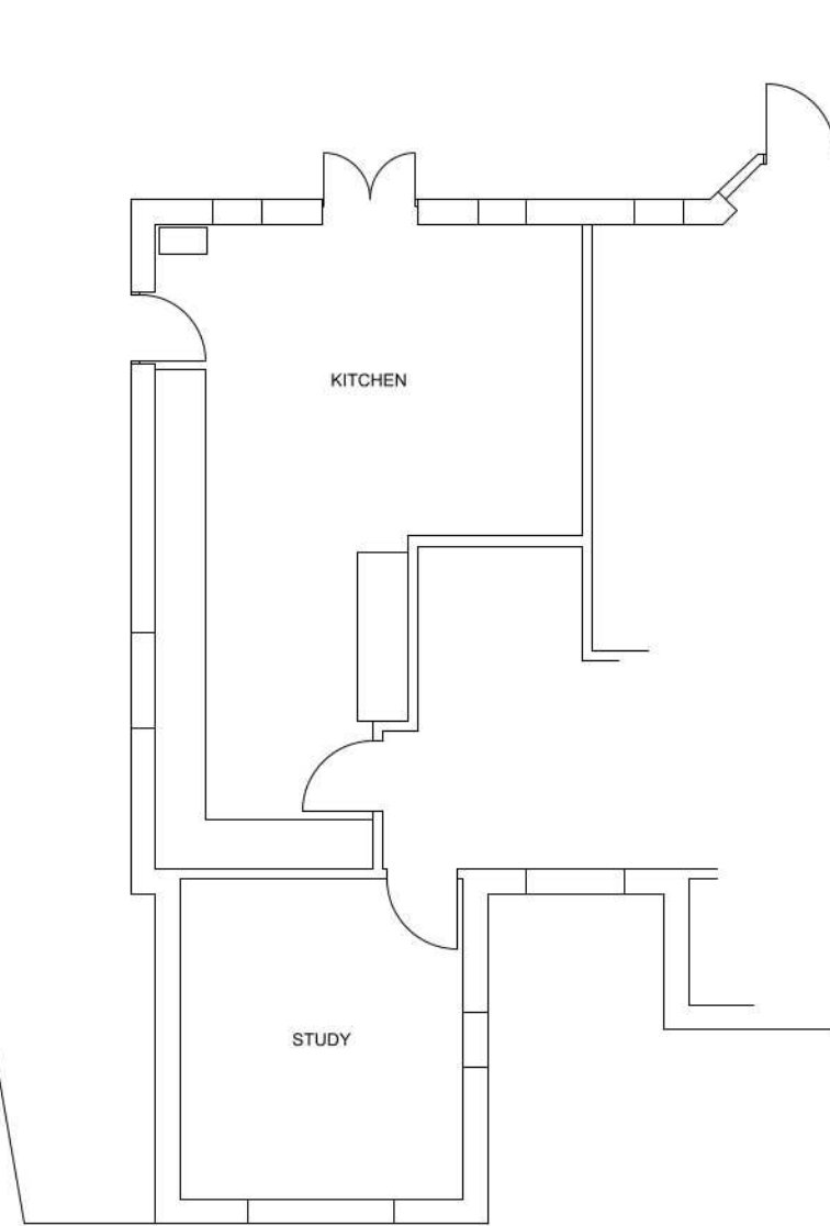
EXISTING GROUND FLOOR PLAN SCALE 1:100 @ a3
