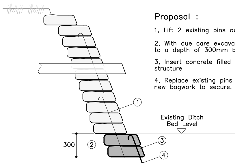
Headwall Section Outfall to side of Ditch
