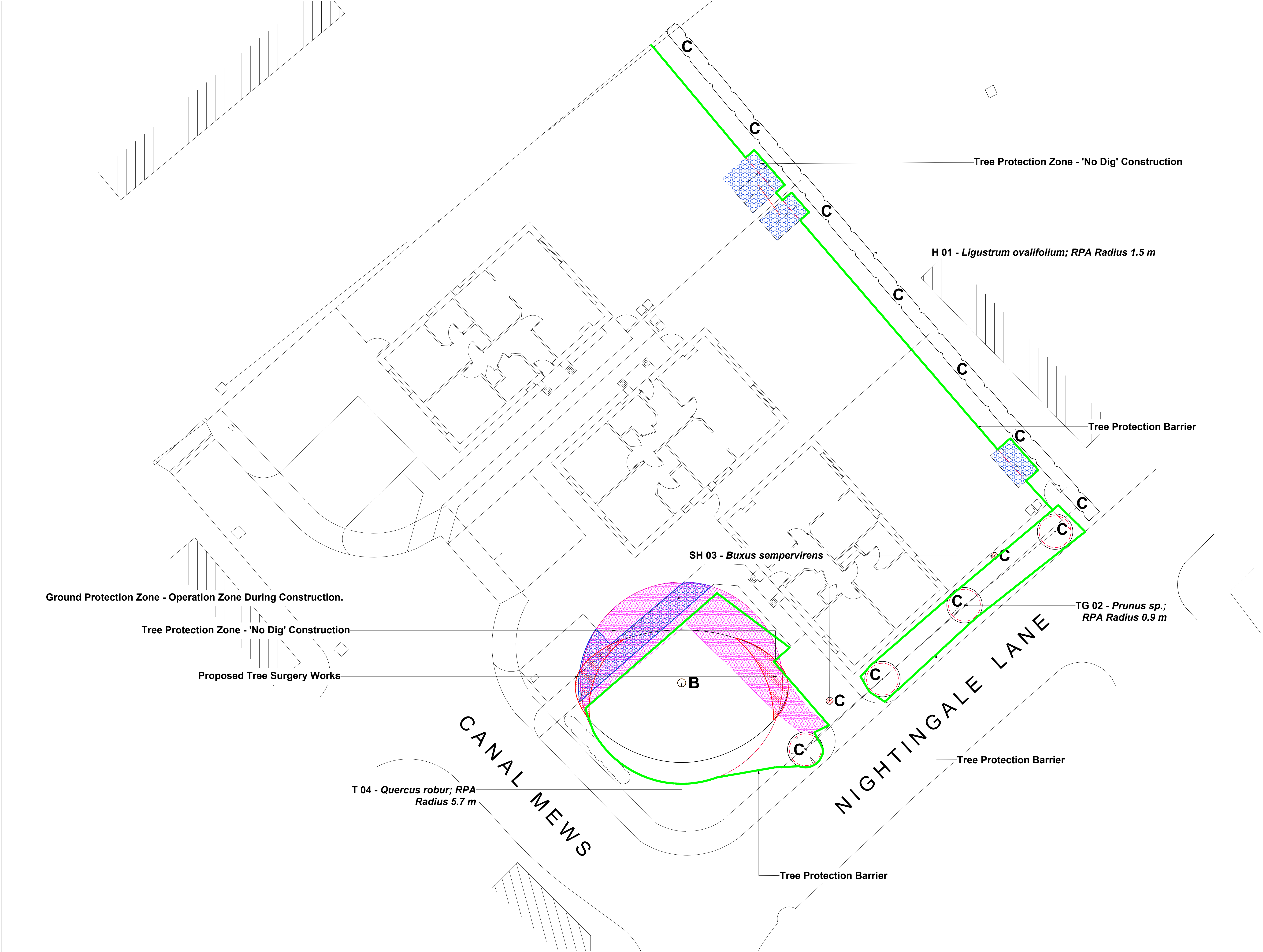
Drawing No. 02 - Tree Retention and Protection Plan Land to the East of Barn Rise, Barnham
