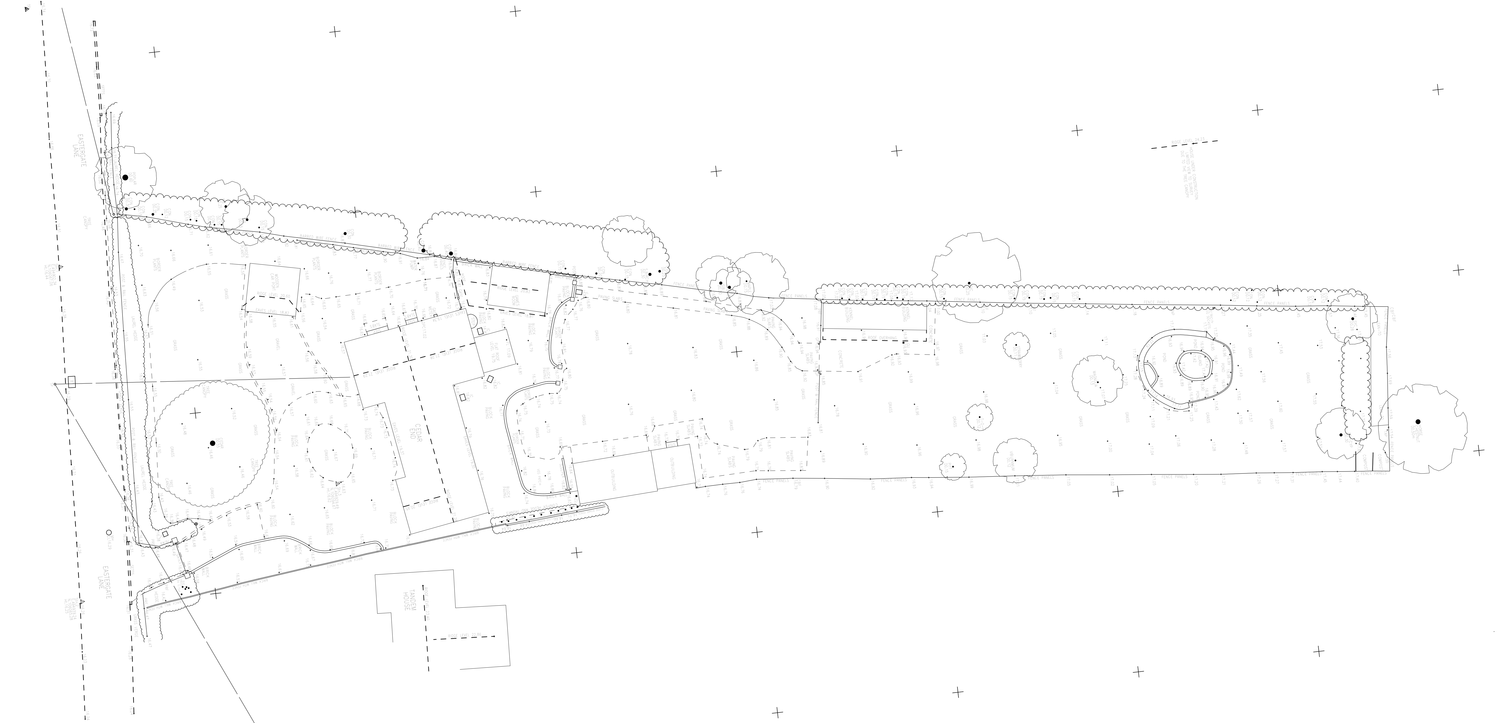
Existing Topographic Site Plan 1:200
