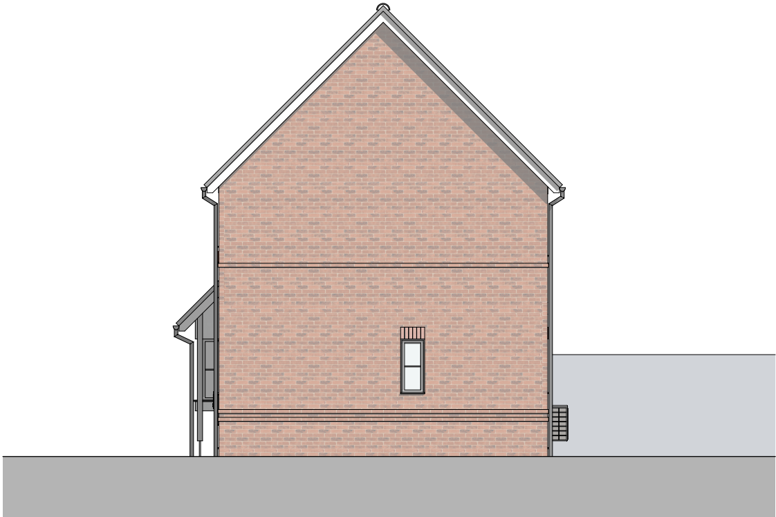
Side Elevation 1:100
