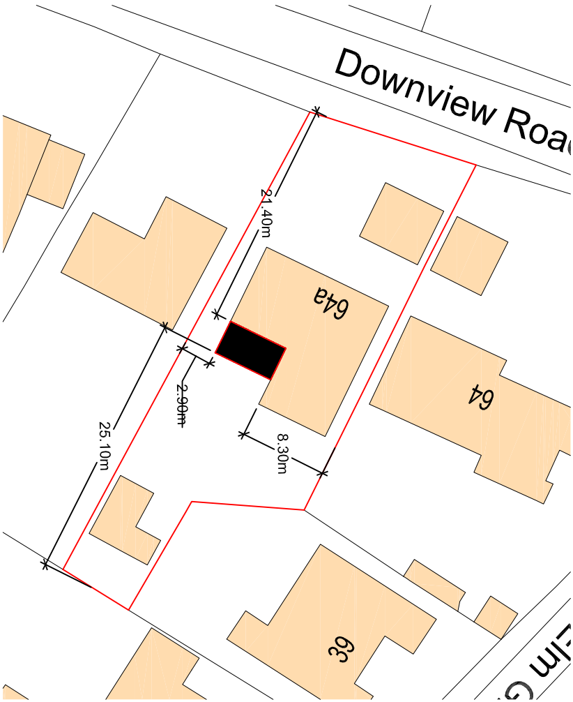
Site Plan 0m 5m 10m 15m 20m 1:500 Scale bar
