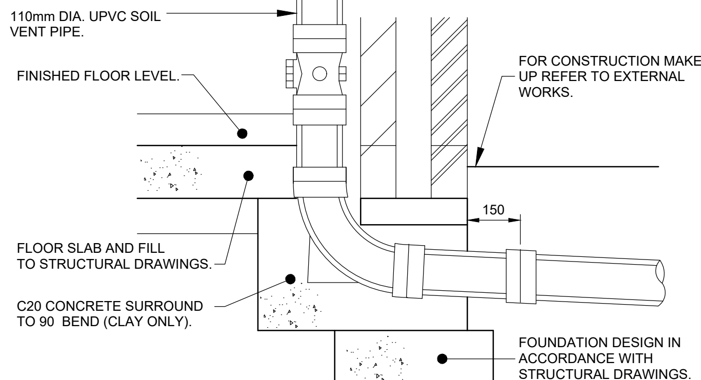
SOIL VENT PIPE CONNECTION
