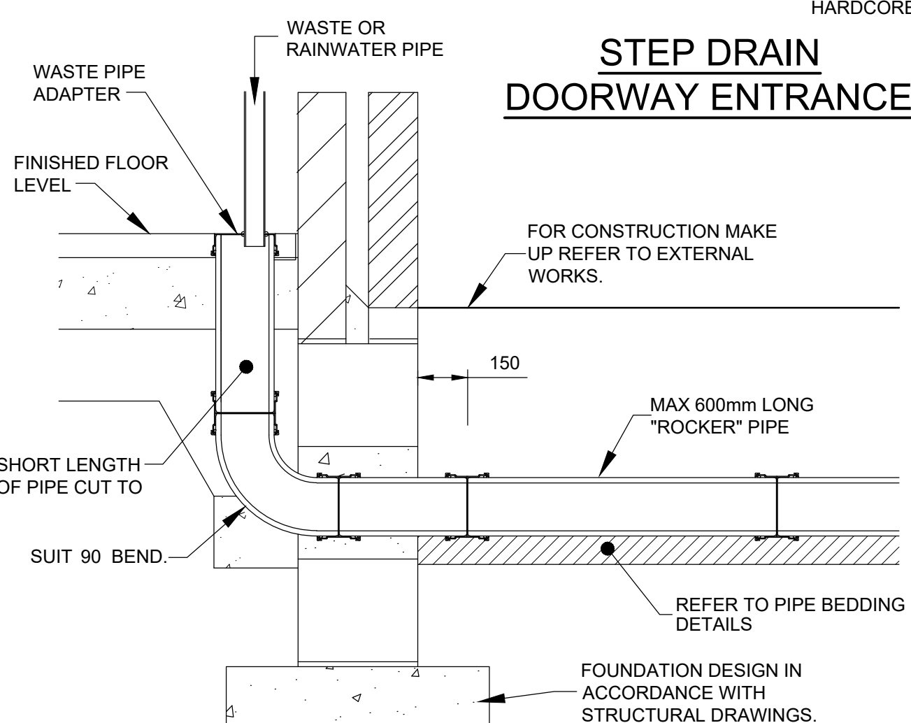
WASTE PIPE DIRECT CONNECTION DETAIL
