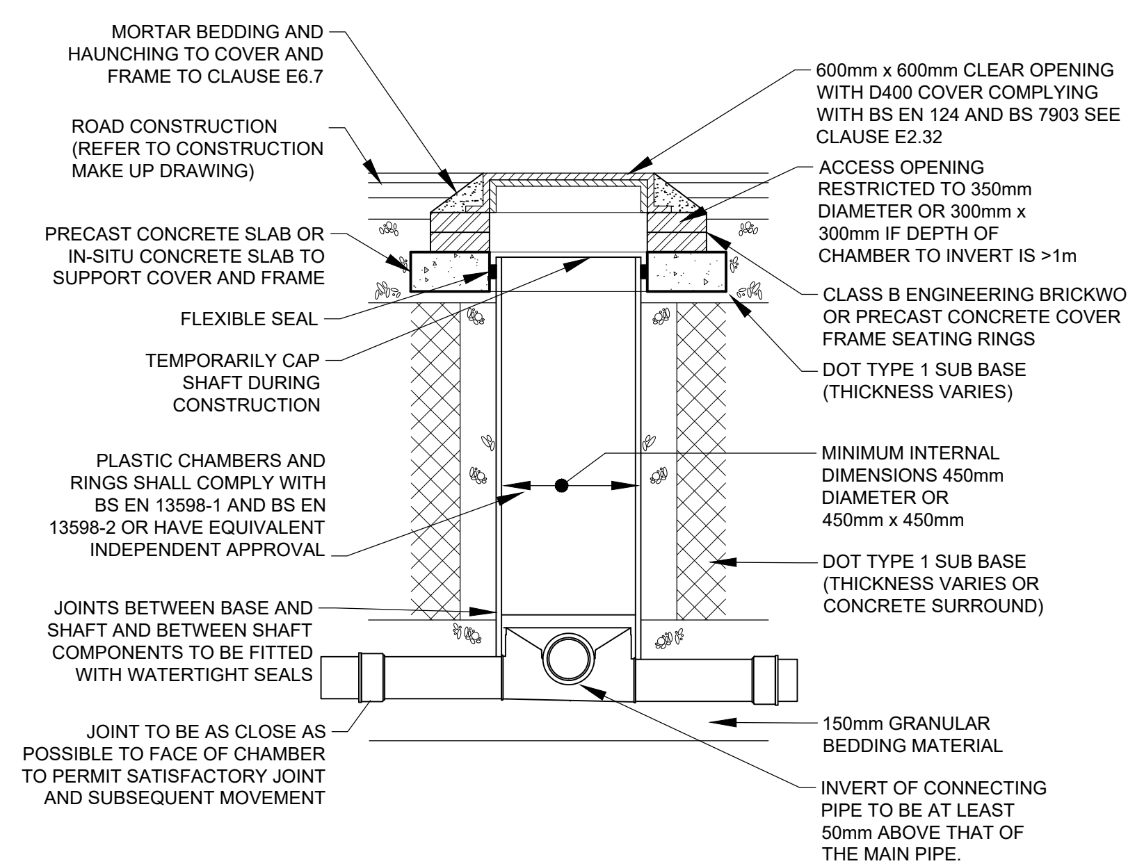
TYPICAL INSPECTION CHAMBER DETAIL - TYPE 3
