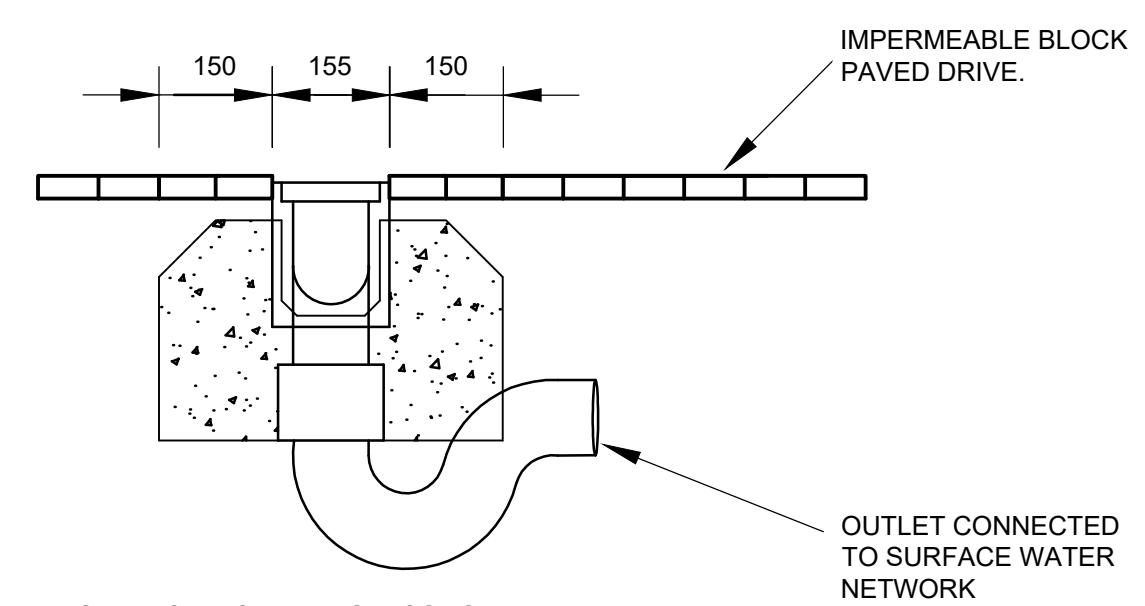
TYPICAL INSPECTION CHAMBER DETAIL - TYPE 3
