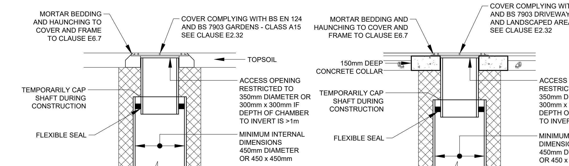
TYPICAL INSPECTION CHAMBER - TYPE 4
