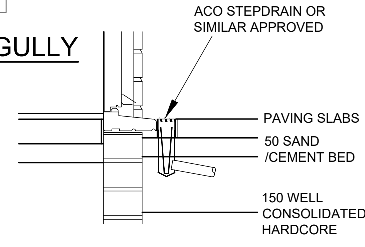
STEP DRAIN DOORWAY ENTRANCE
