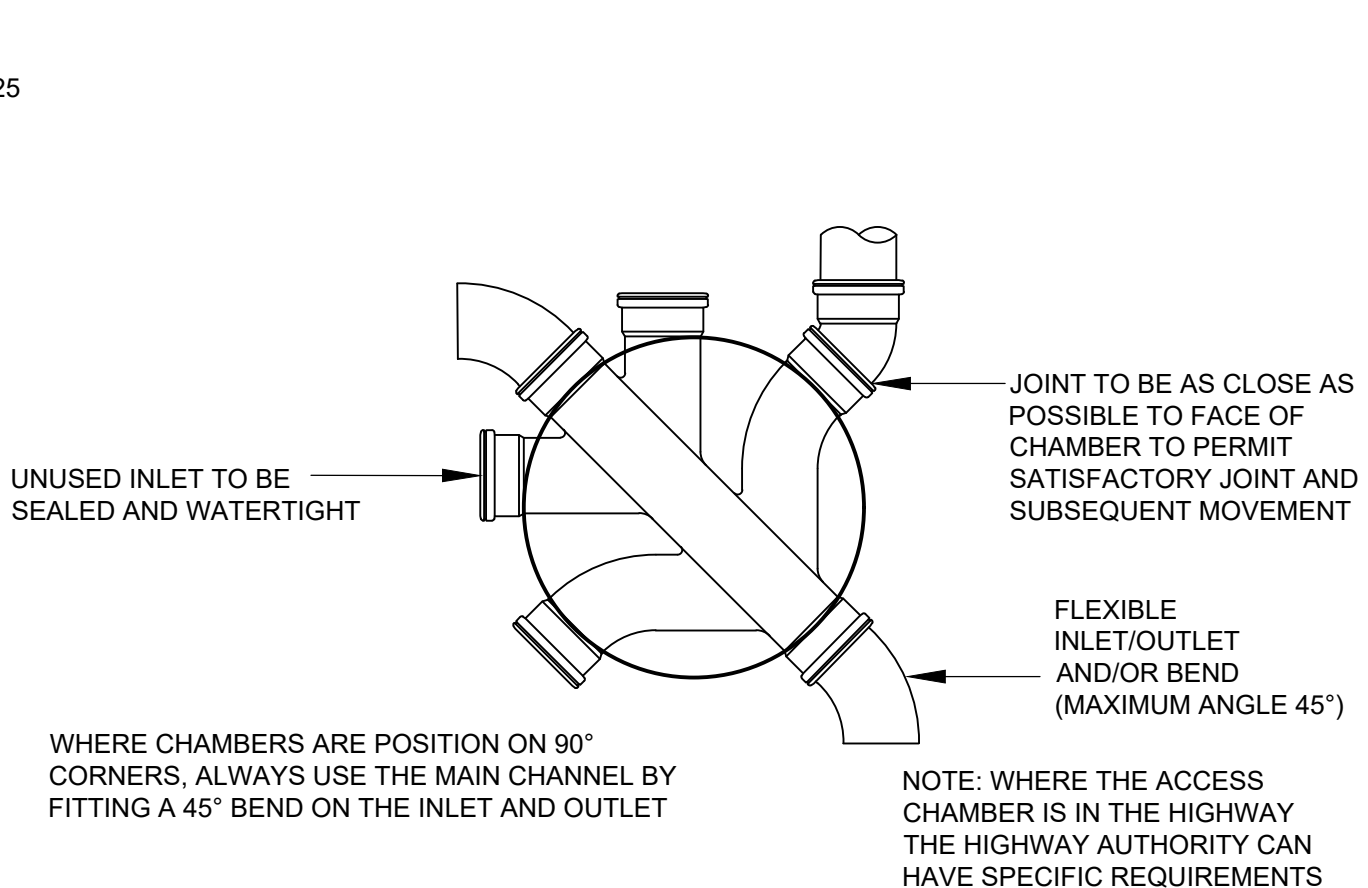
TYPICAL INSPECTION CHAMBER BASE LAYOUT - TYPE 3
