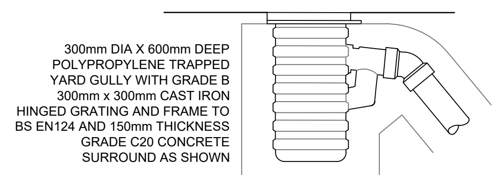
ULTRA-RIB YARD GULLY
