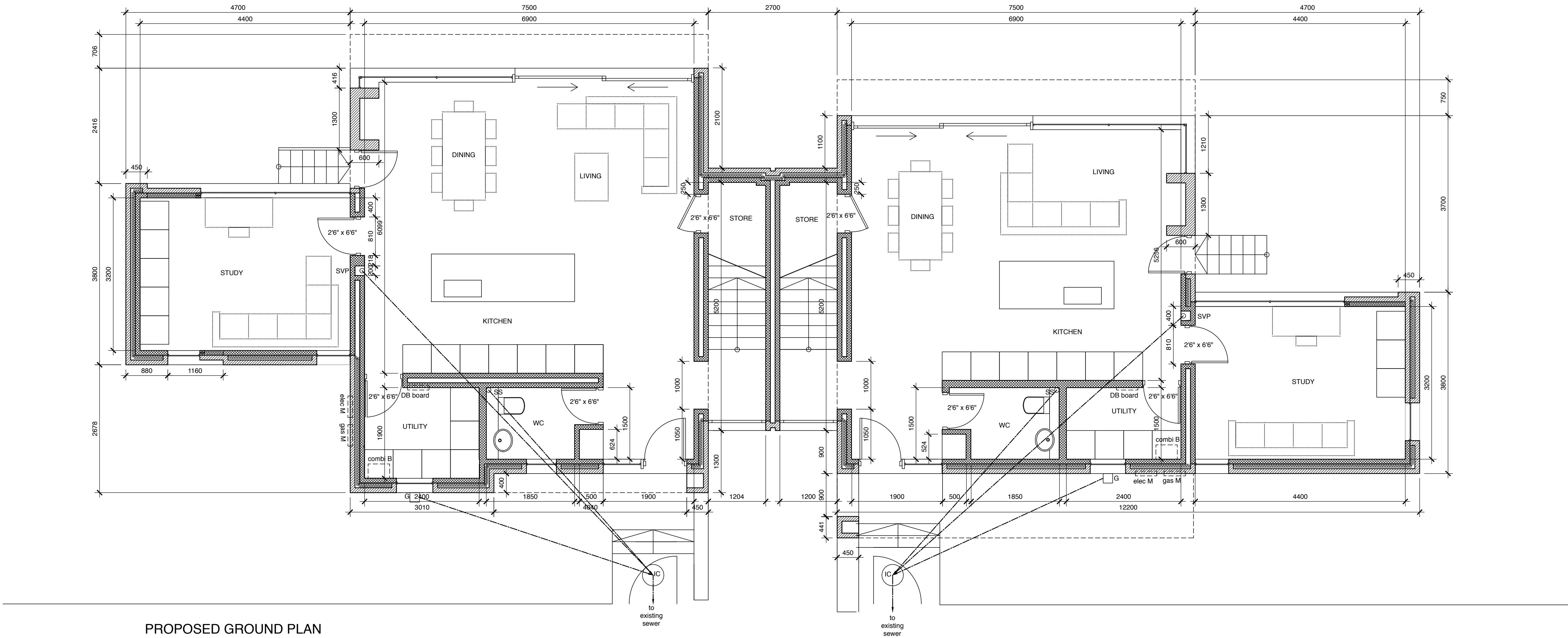
PROPOSED GROUND PLAN
